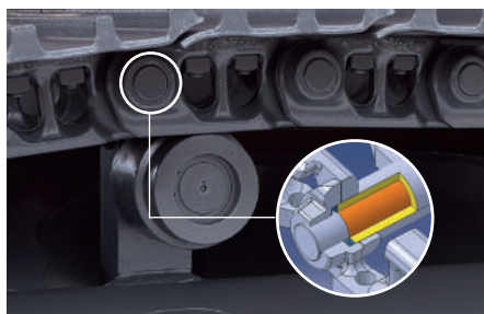
Tracks The chain is composed of self-lubricating sealed links isolated from all external contamination. The tracks are locked by mechanically bolted pins.
